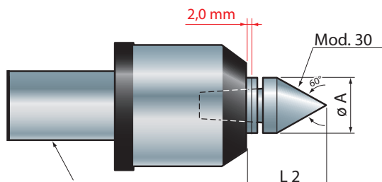
Attacco Connector / Anschluss
