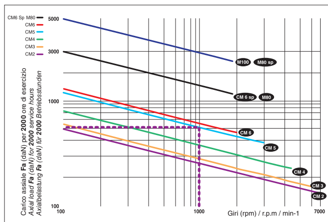
MOD. M Carico assiale / Axial load / Axialbelastung
